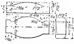
Fig. 5145. Stop-wedge.
